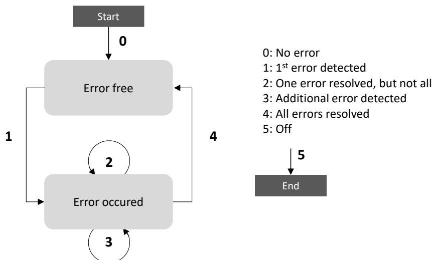
Figure 25 – EMCY error state machine
