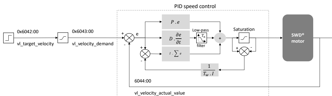
Figure 38 – Speed controller
